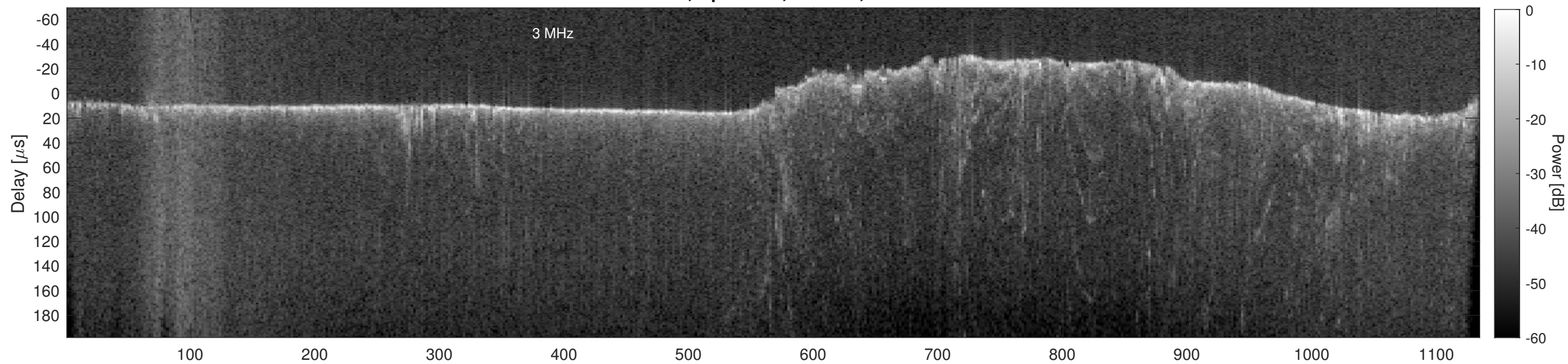
Orbit 13470, Cluttergram
