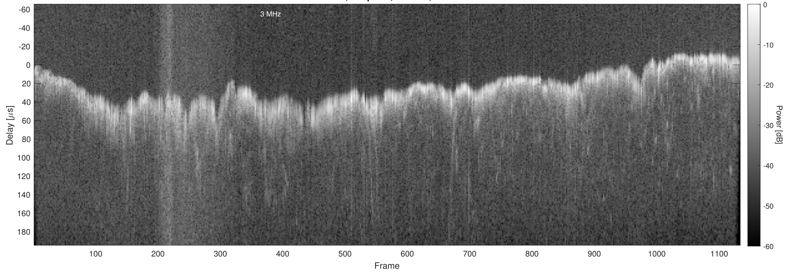
Orbit 13471, Chapman, Window, Channel 2
