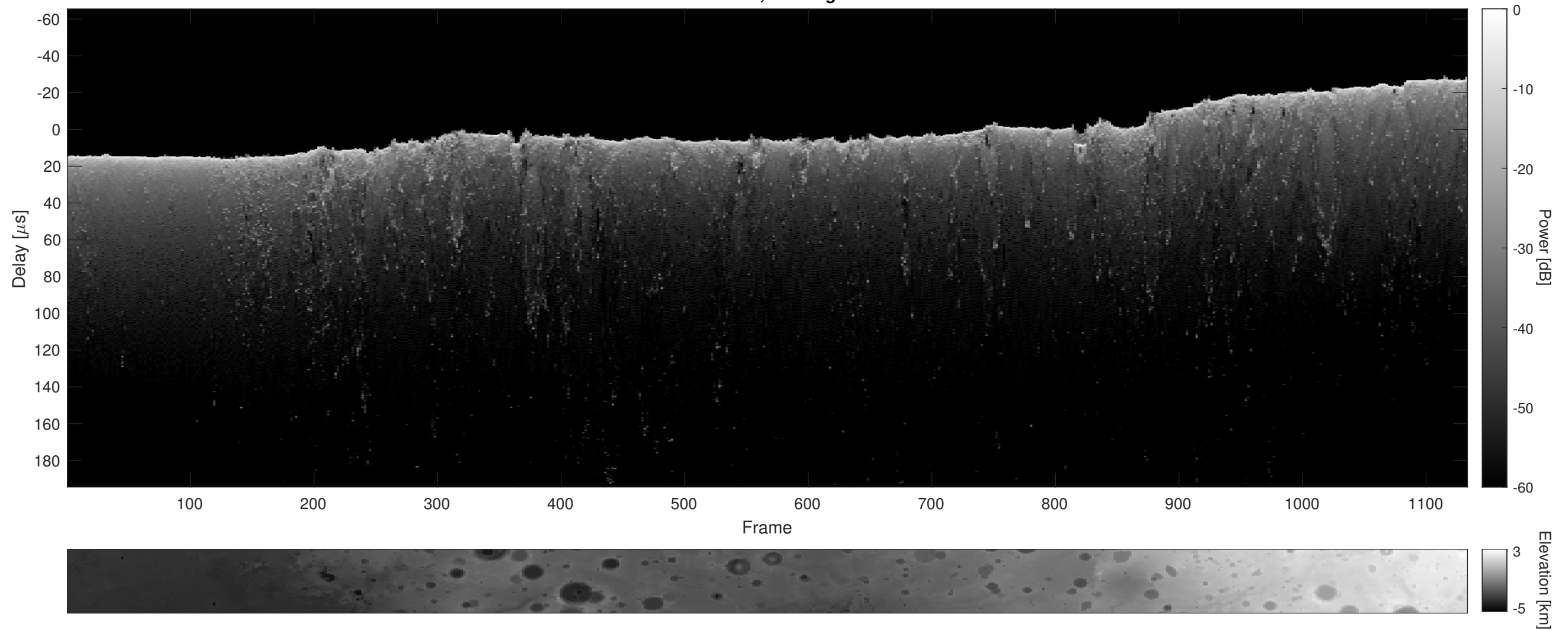
Orbit 13471, Cluttergram
