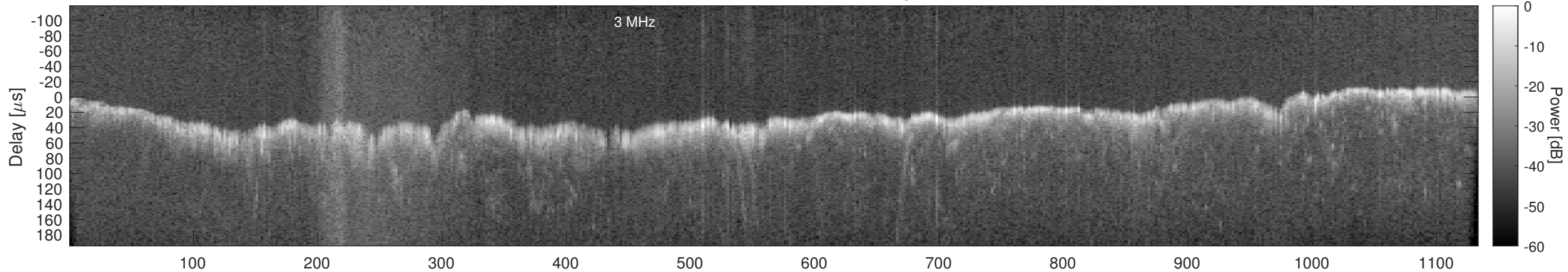
Orbit 13471, Window, Channel 2, Optimized
