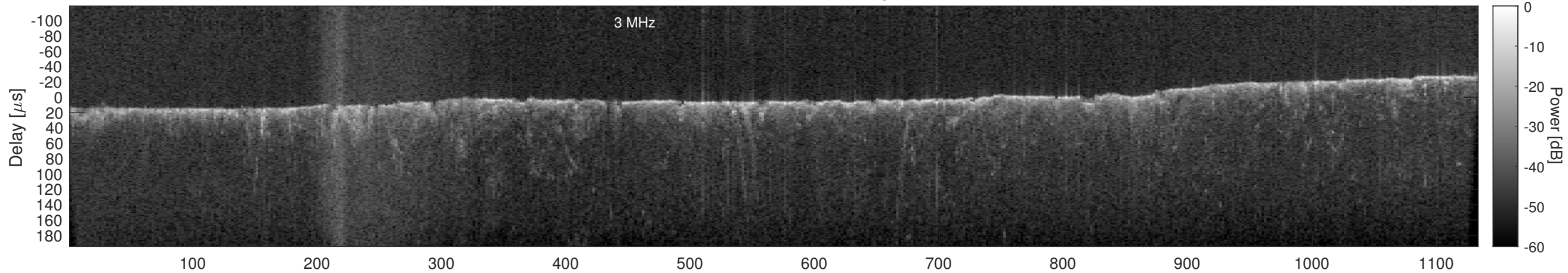
Orbit 13471, Cluttergram
