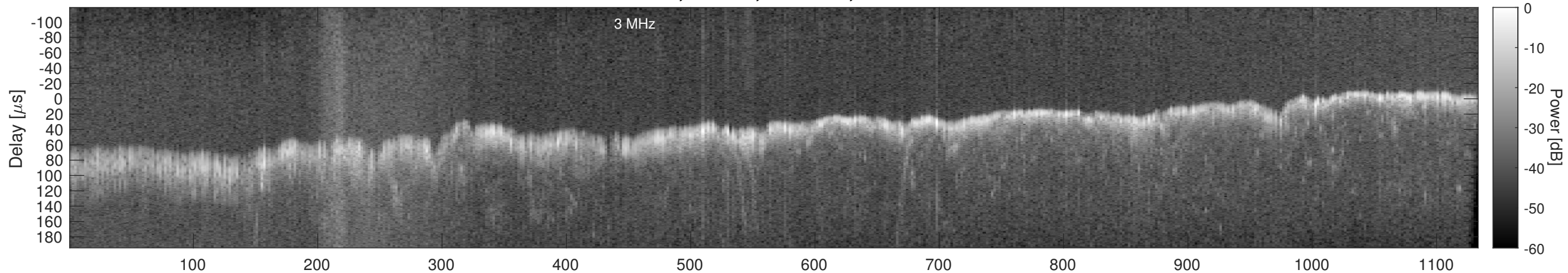
Orbit 13471, Window, Channel 2, Chapman
