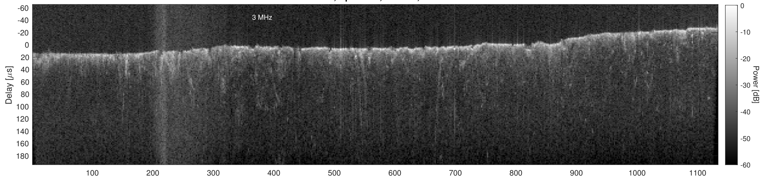
Orbit 13471, Cluttergram
