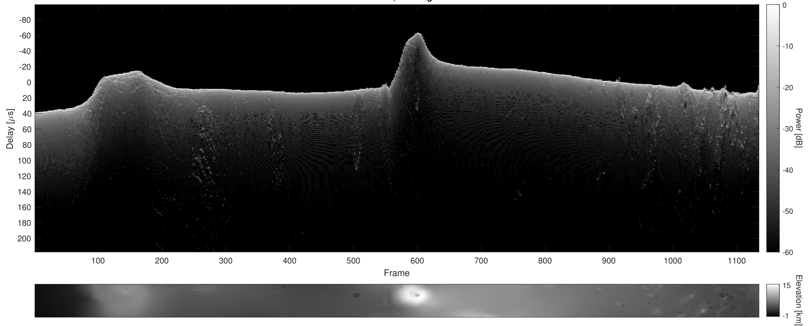
Orbit 13472, Cluttergram
