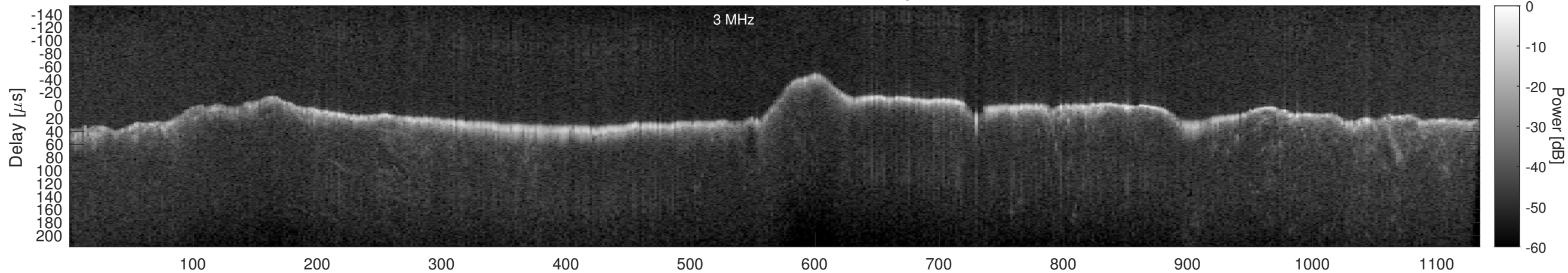
Orbit 13472, Window, Channel 2, Optimized
