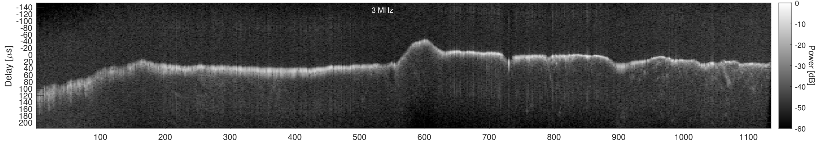
Orbit 13472, Window, Channel 2, Chapman
