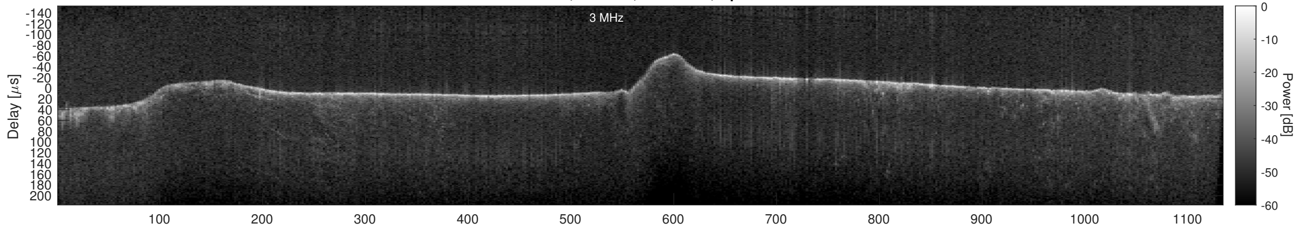
Orbit 13472, Cluttergram
