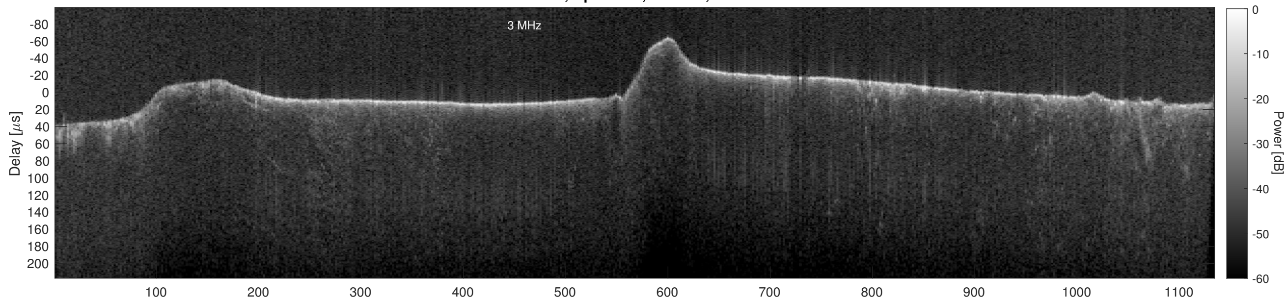
Orbit 13472, Cluttergram
