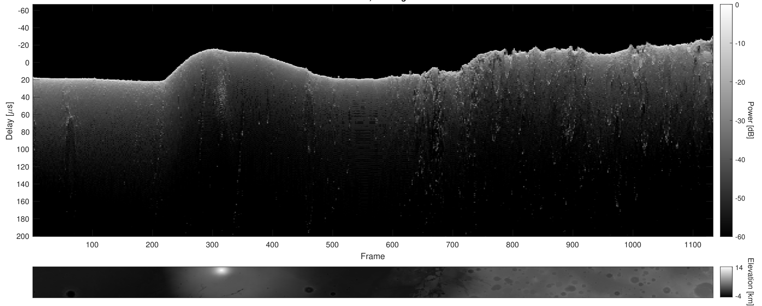
Orbit 13473, Cluttergram
