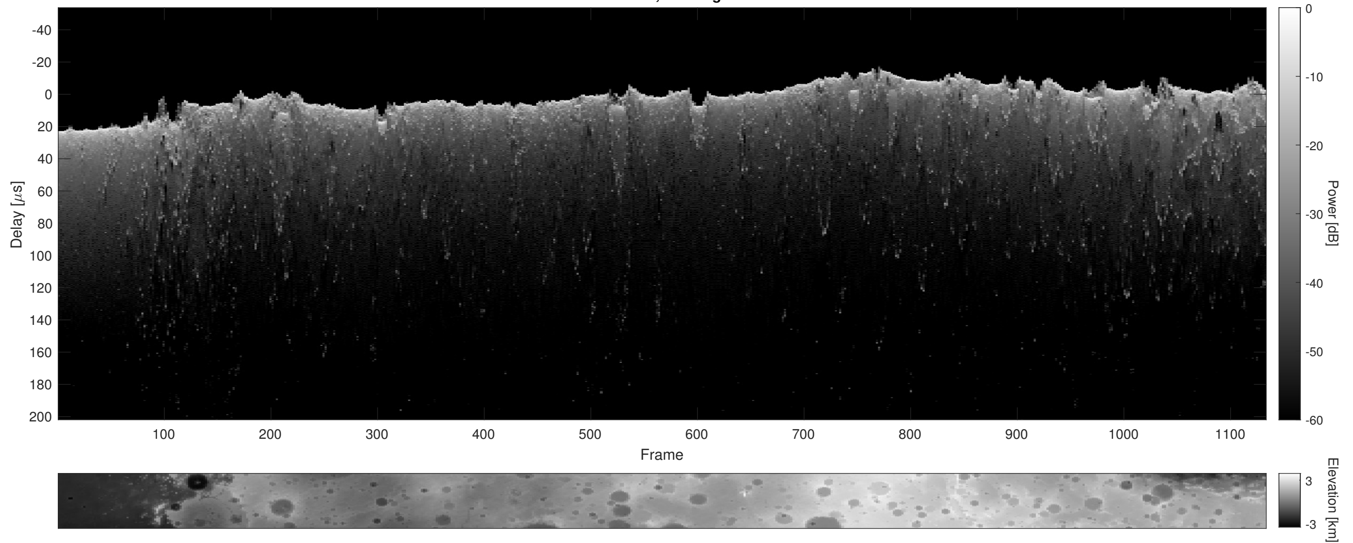
Orbit 13474, Cluttergram
