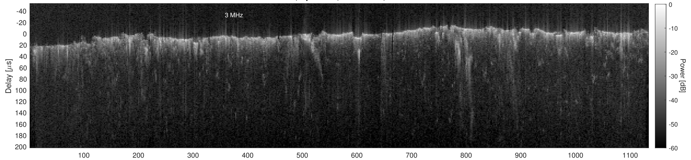
Orbit 13474, Cluttergram
