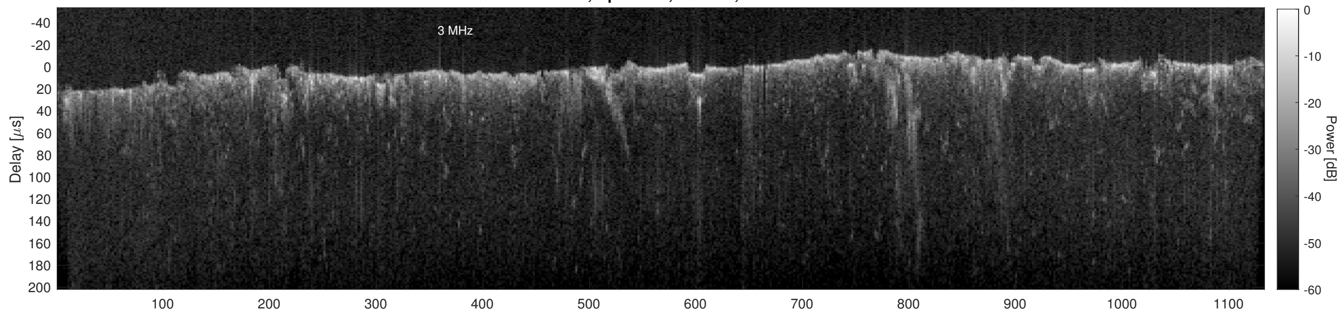
Orbit 13474, Cluttergram
