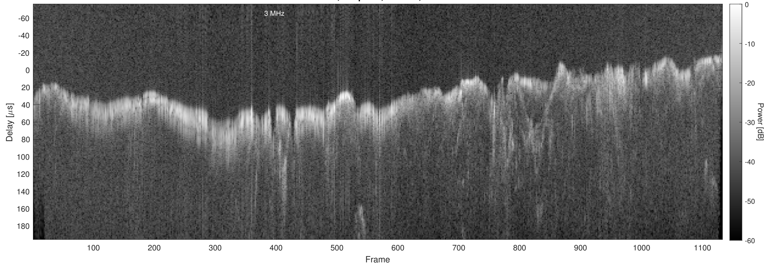
Orbit 13476, Chapman, Window, Channel 2
