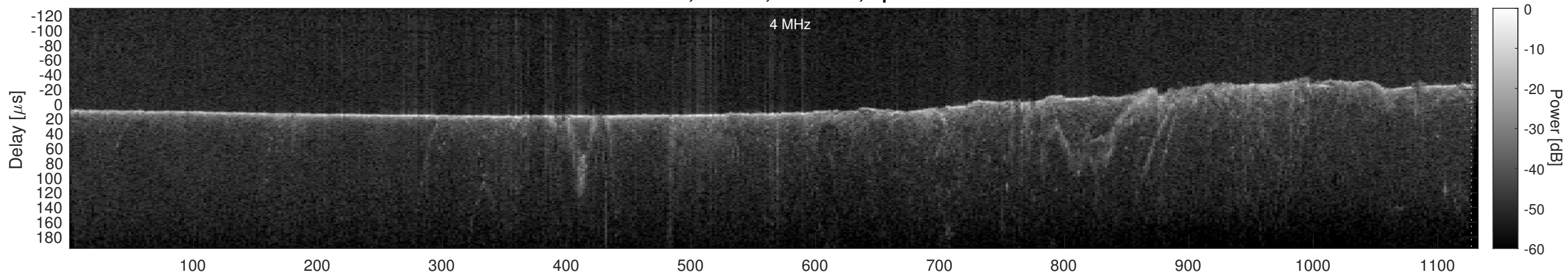
Orbit 13476, Cluttergram
