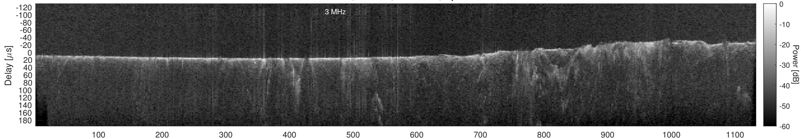
Orbit 13476, Cluttergram
