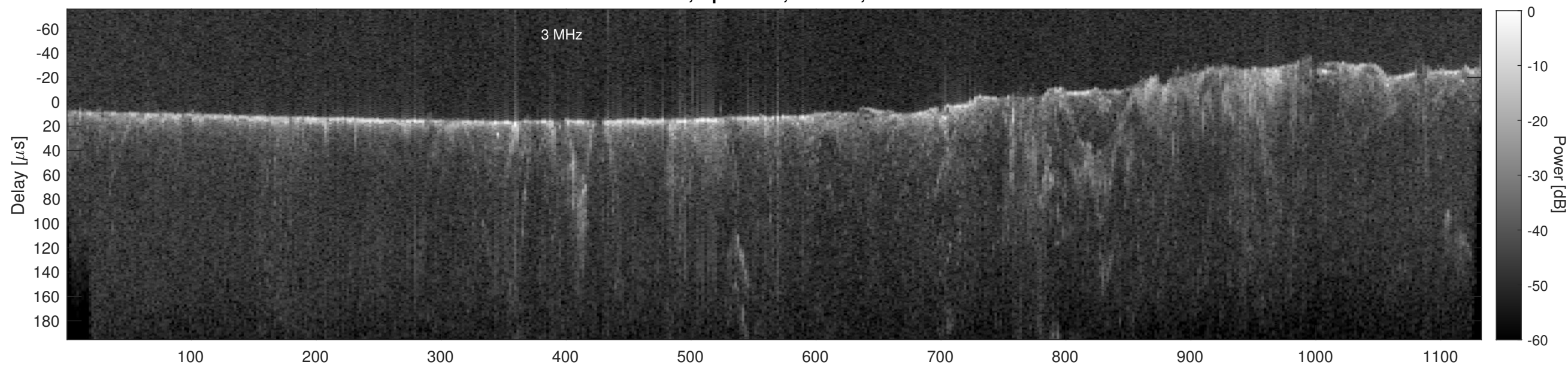
Orbit 13476, Cluttergram
