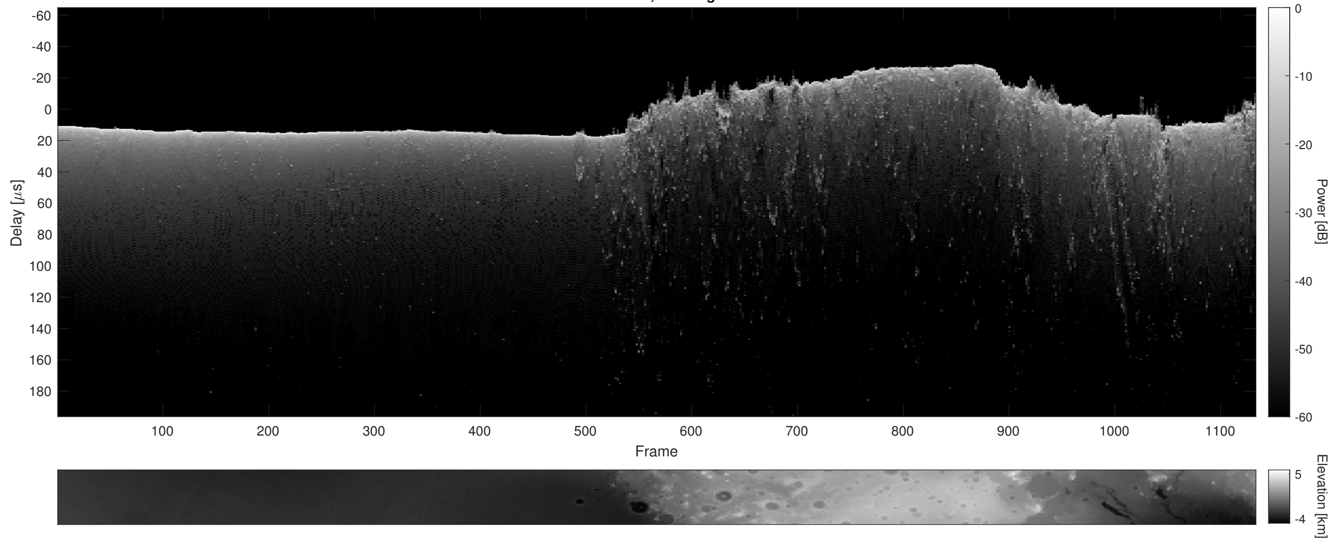
Orbit 13477, Cluttergram
