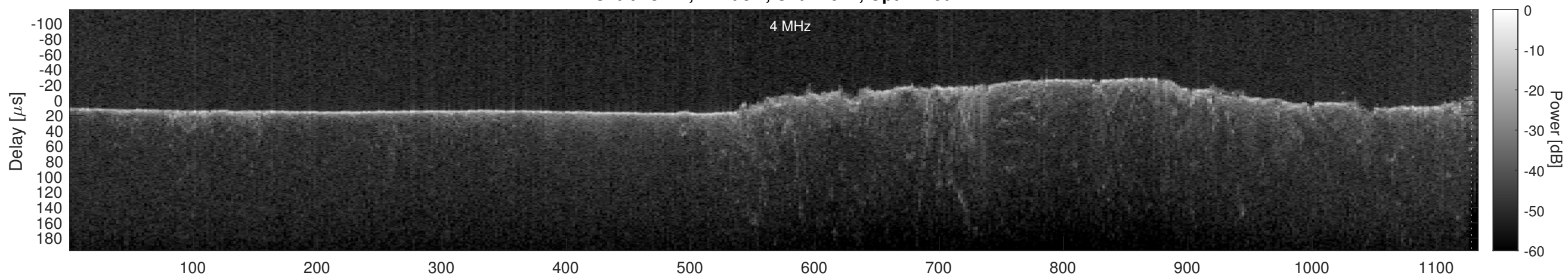
Orbit 13477, Cluttergram
