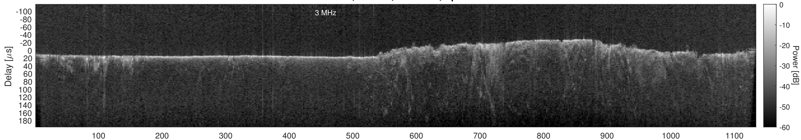
Orbit 13477, Cluttergram
