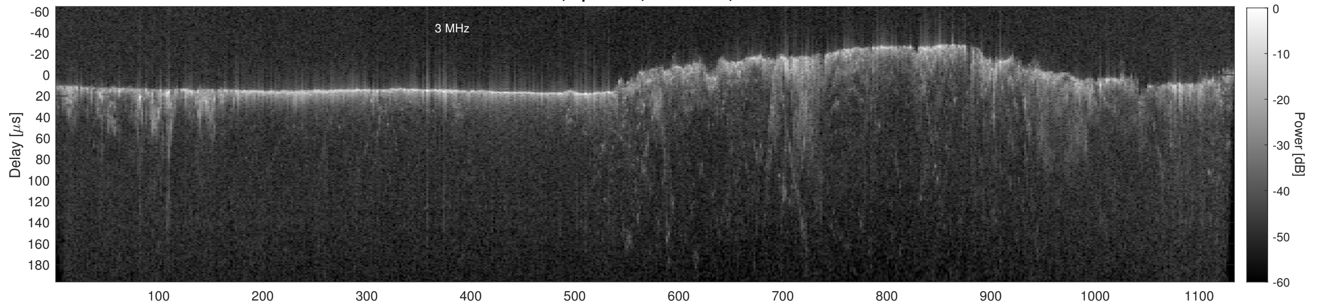
Orbit 13477, Cluttergram
