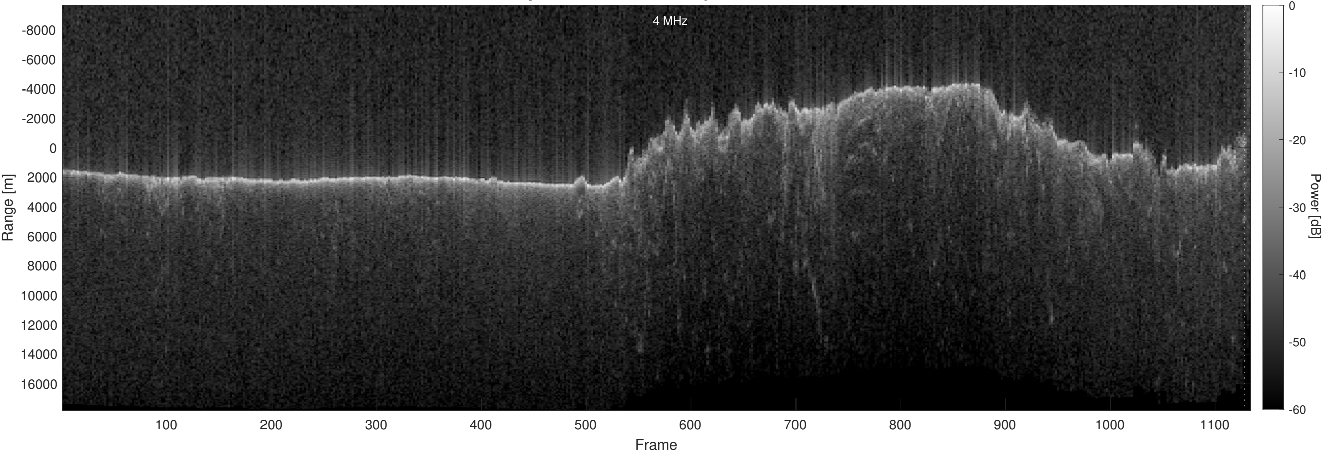
Orbit 13477, Optimized, No Window, Depth-Corrected, Channel 2
