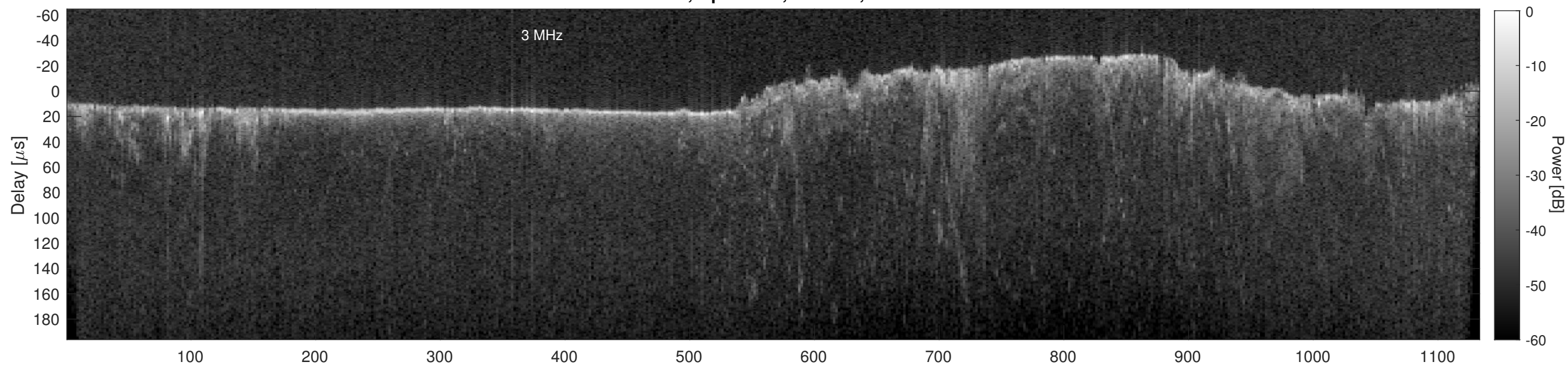
Orbit 13477, Cluttergram
