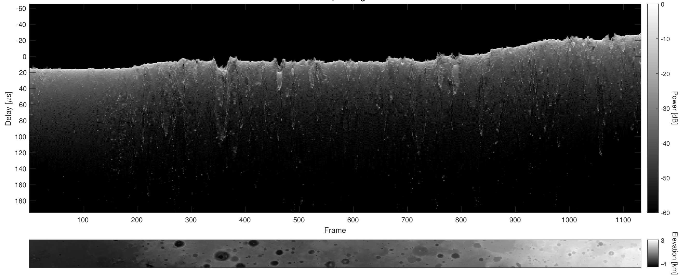
Orbit 13478, Cluttergram
