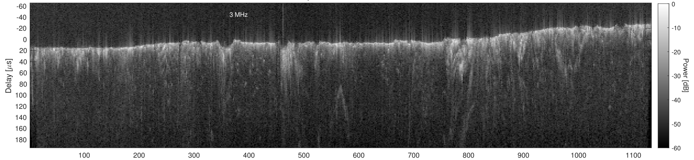
Orbit 13478, Cluttergram
