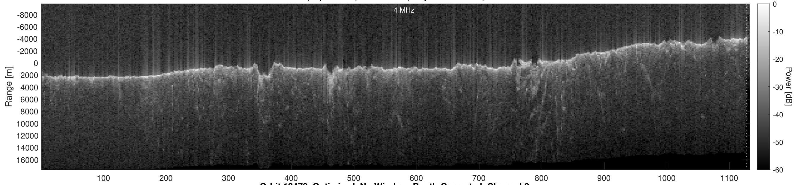
Orbit 13478, Optimized, No Window, Depth-Corrected, Channel 2
