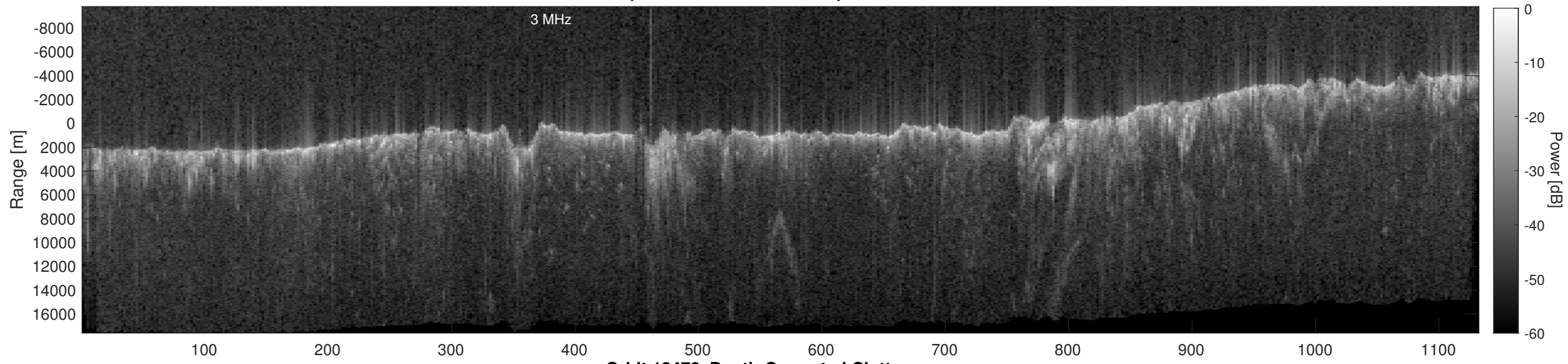
Orbit 13478, Depth-Corrected Cluttergram
