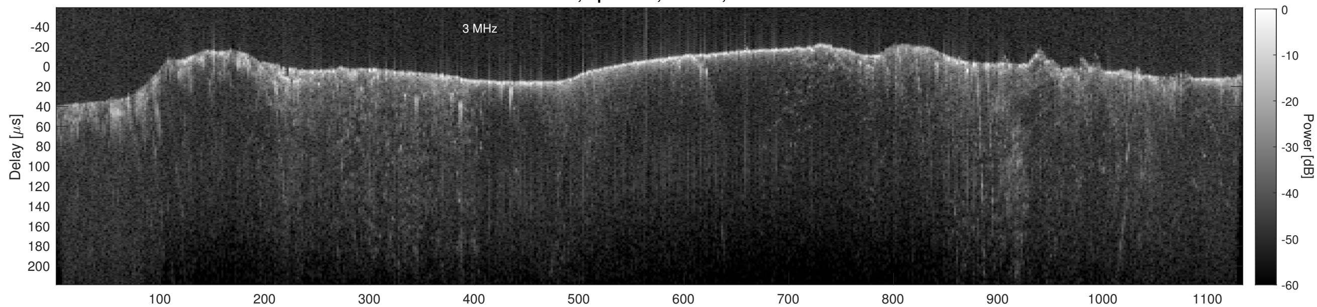
Orbit 13479, Cluttergram
