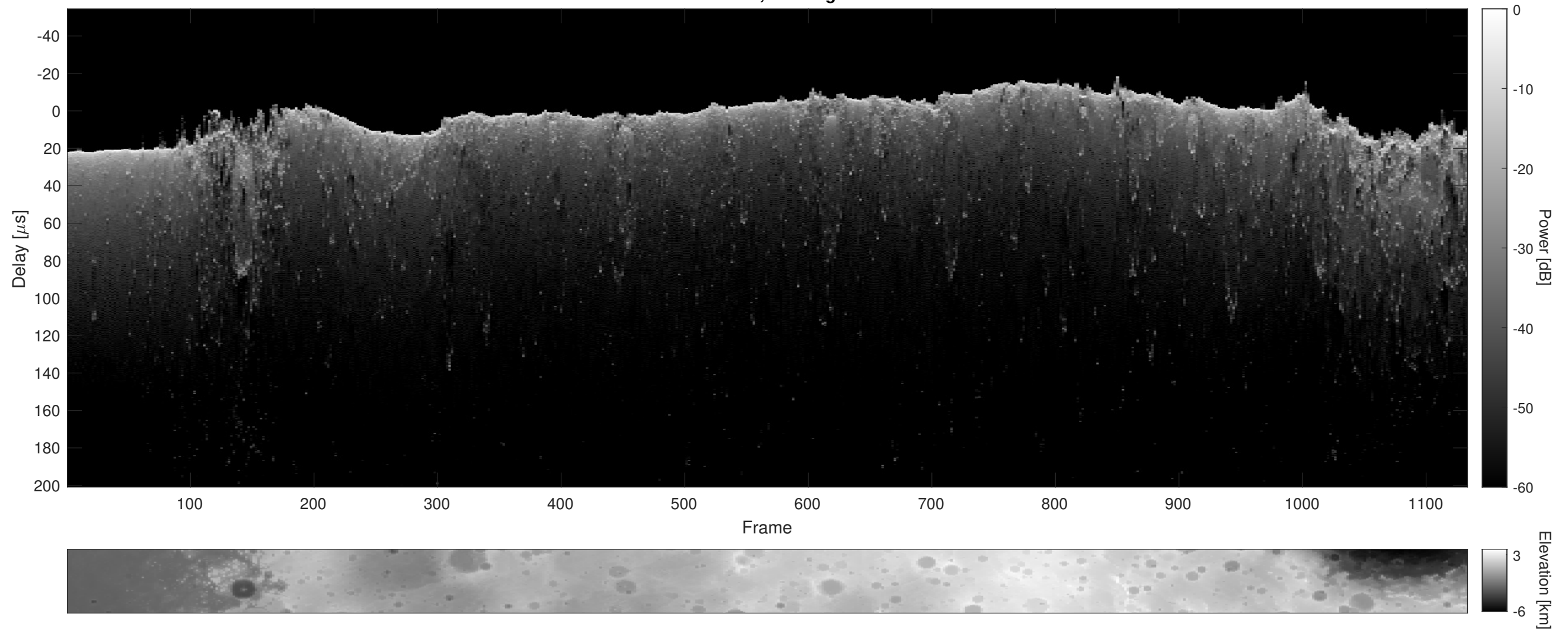
Orbit 13481, Cluttergram
