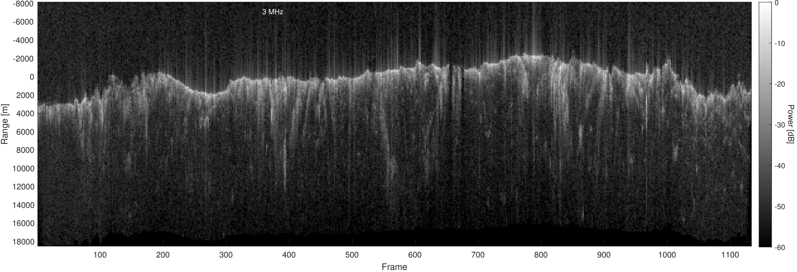
Orbit 13481, Optimized, No Window, Depth-Corrected, Channel 2
