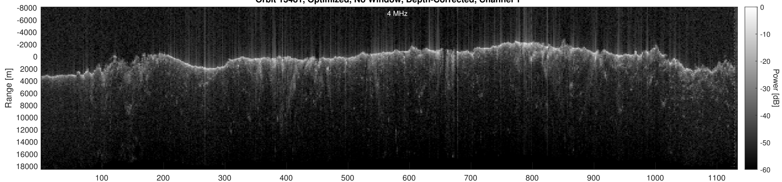
Orbit 13481, Optimized, No Window, Depth-Corrected, Channel 2
