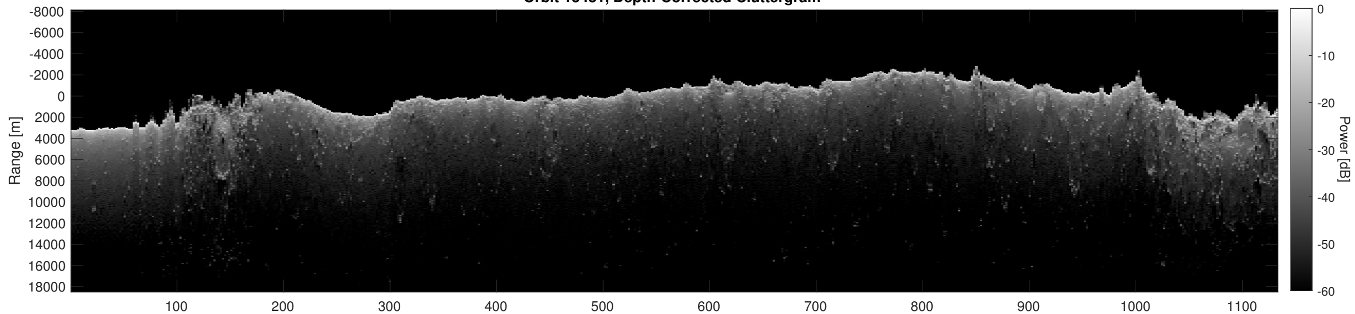
Orbit 13481, Depth-Corrected Cluttergram
