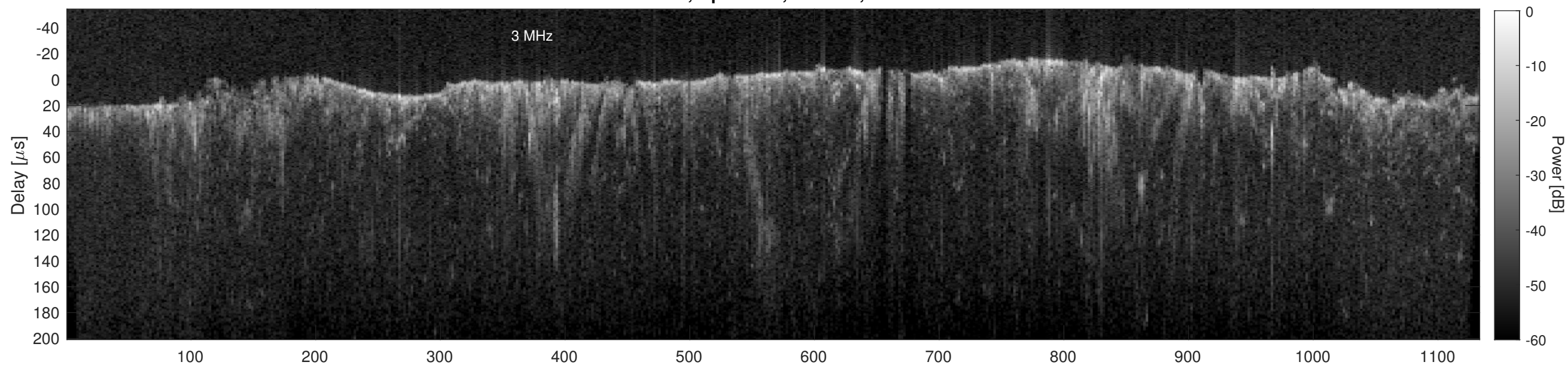
Orbit 13481, Cluttergram
