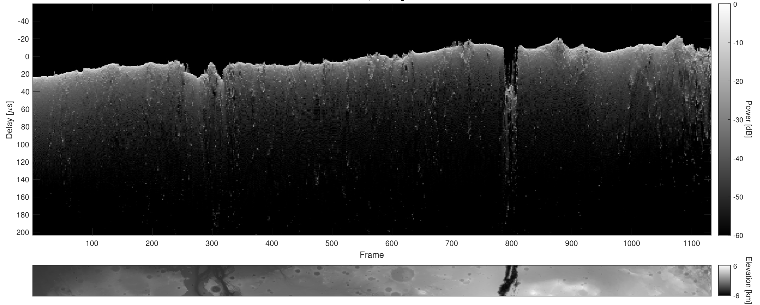
Orbit 13482, Cluttergram
