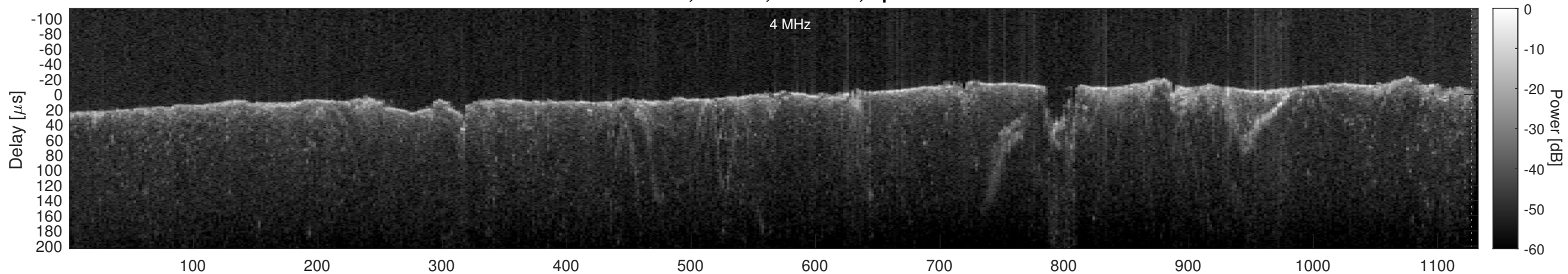
Orbit 13482, Cluttergram
