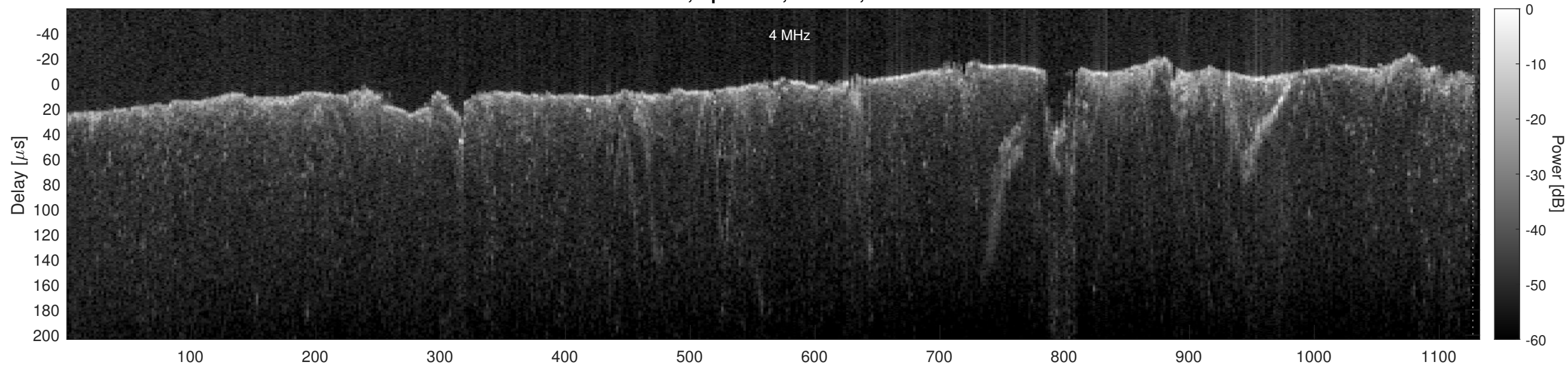
Orbit 13482, Optimized, Window, Channel 2
