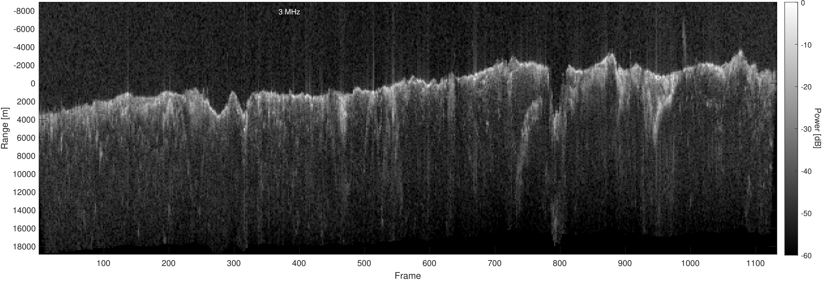
Orbit 13482, Optimized, Window, Depth-Corrected, Channel 2
