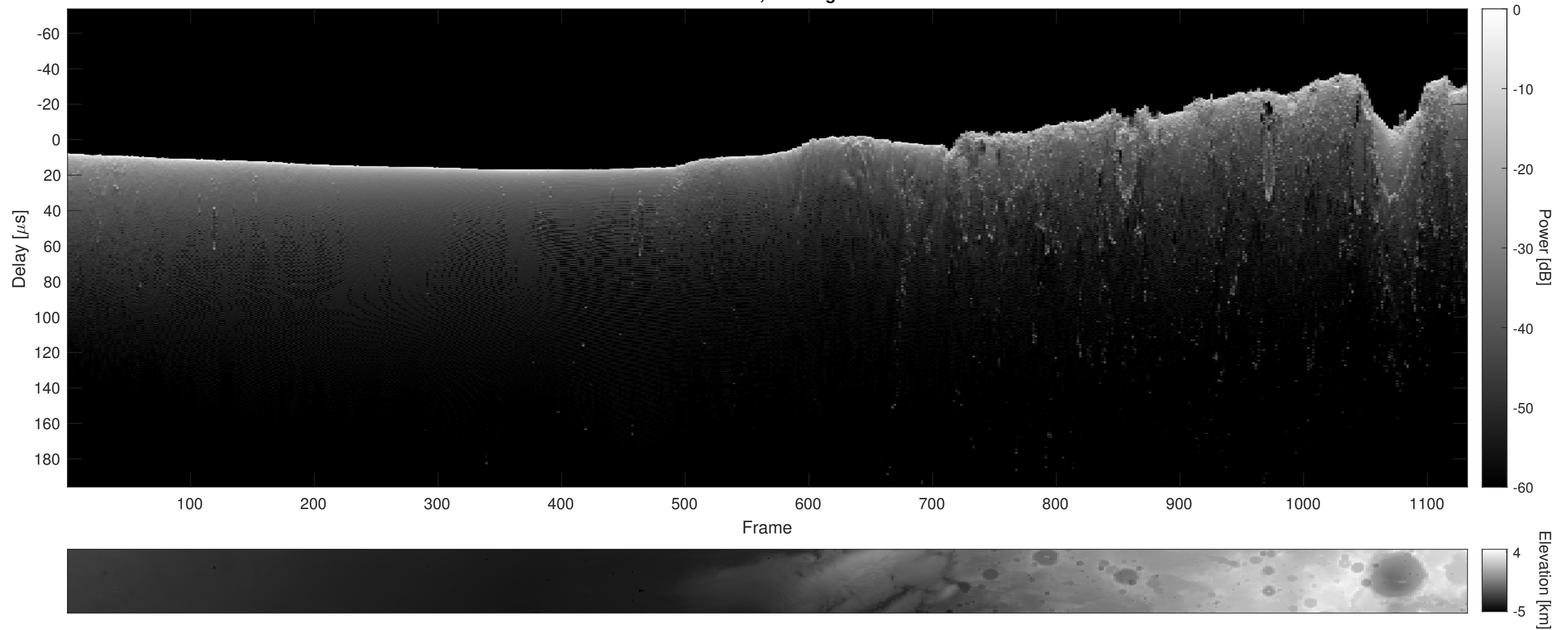
Orbit 13483, Cluttergram
