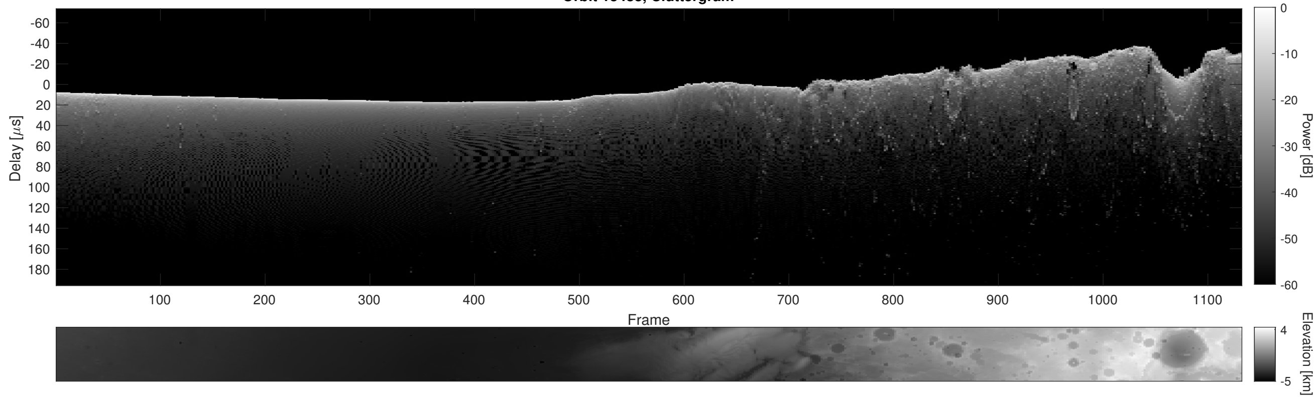
Orbit 13483, Cluttergram
