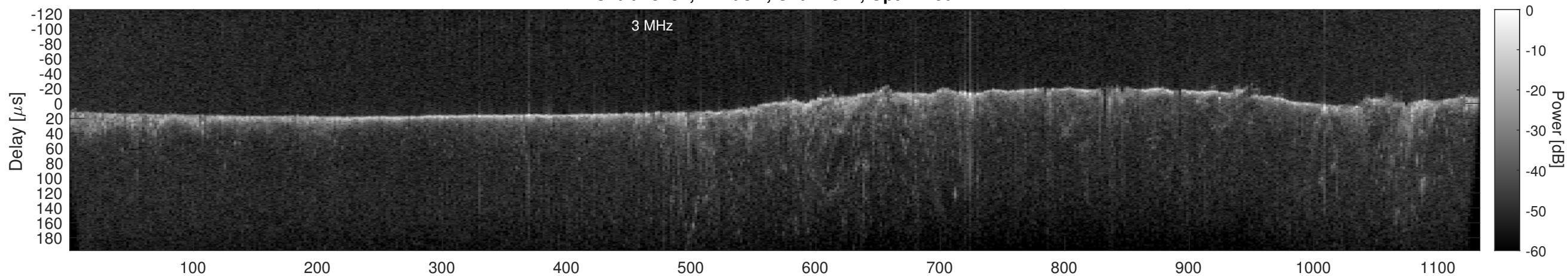
Orbit 13484, Cluttergram
