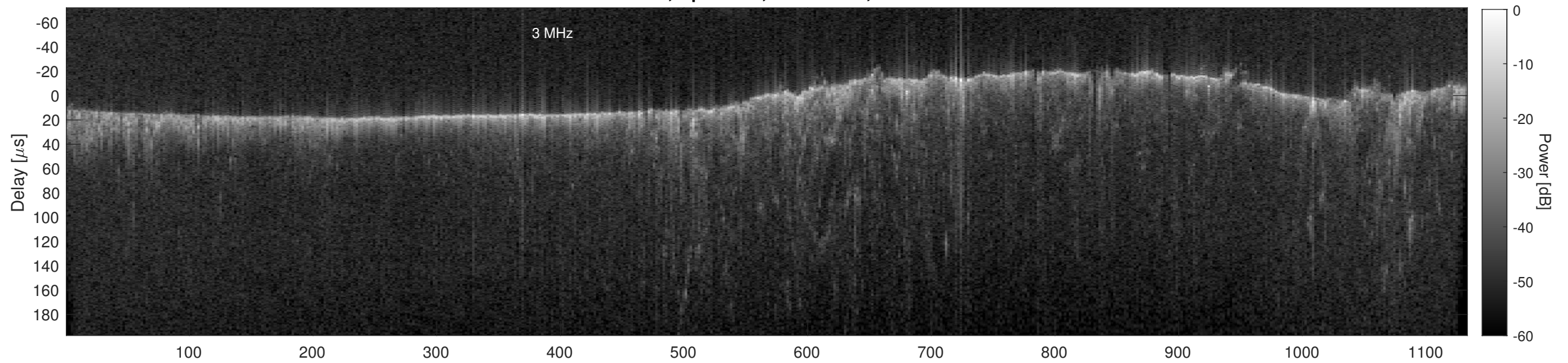
Orbit 13484, Cluttergram
