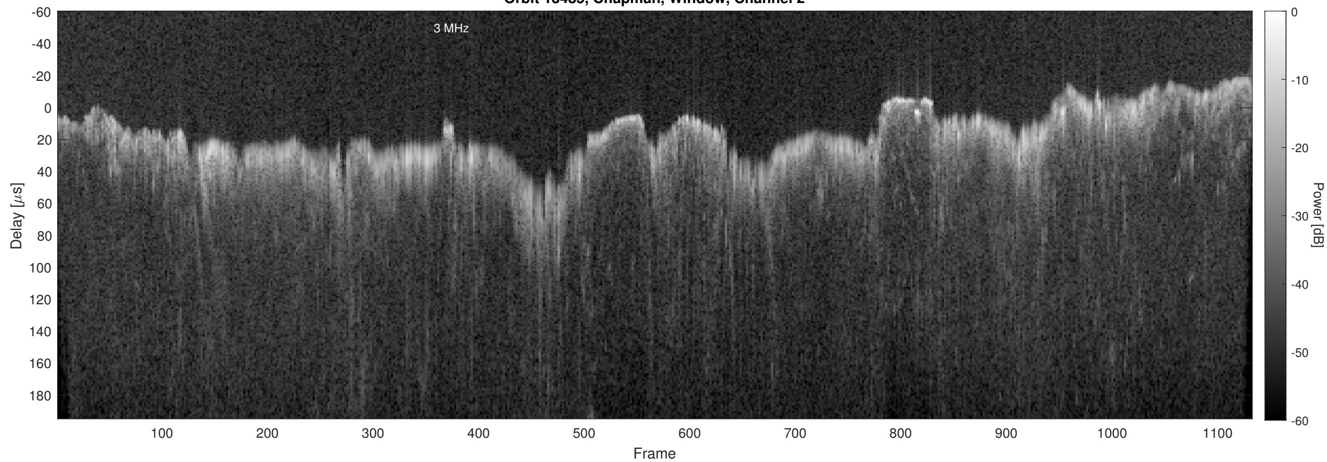
Orbit 13485, Chapman, Window, Channel 2
