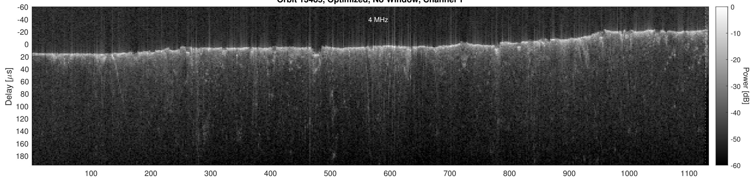
Orbit 13485, Optimized, No Window, Channel 2
