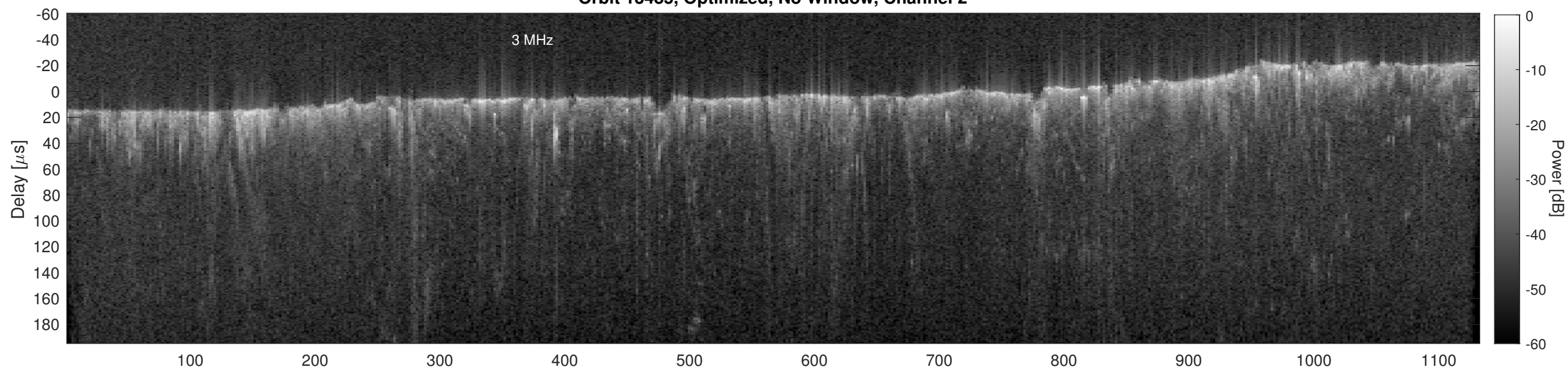
Orbit 13485, Cluttergram
