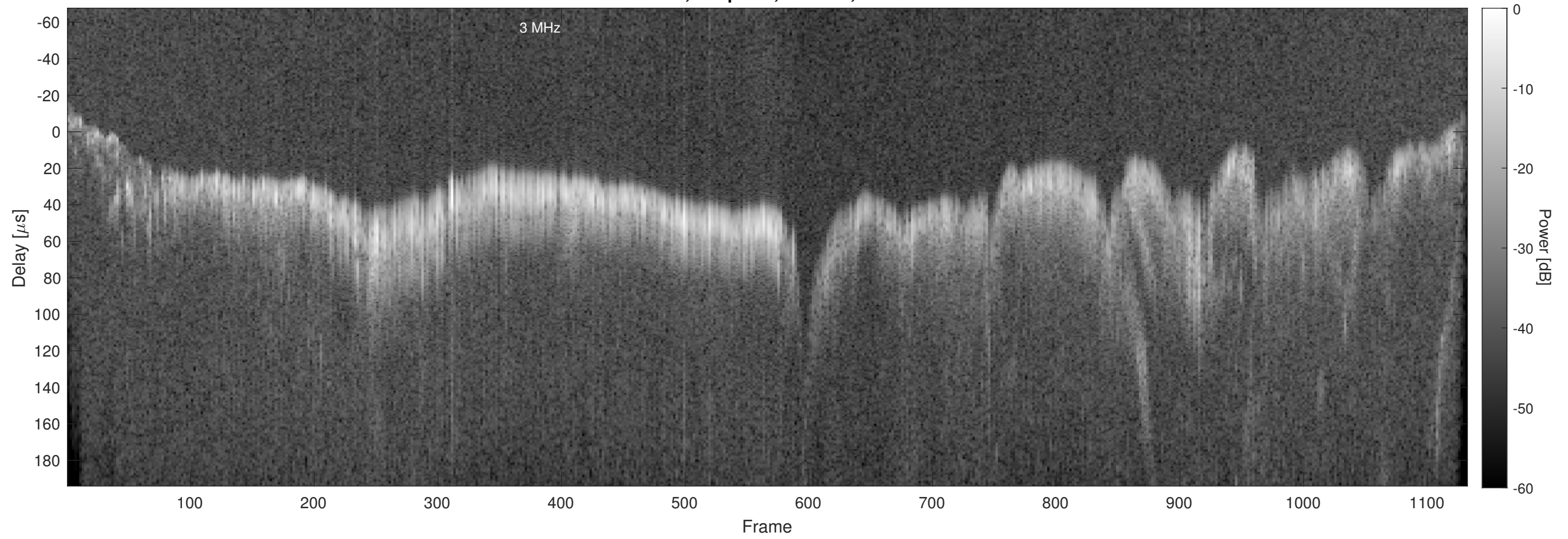
Orbit 13487, Chapman, Window, Channel 2
