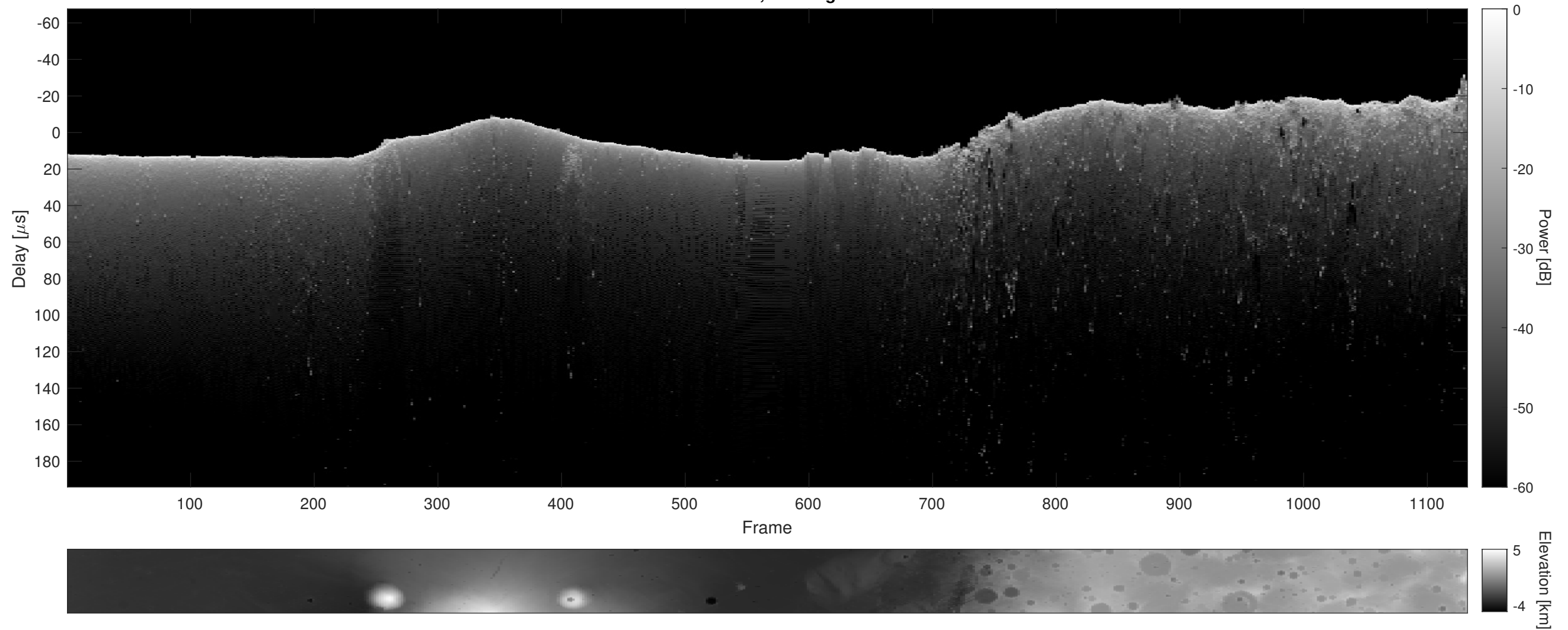
Orbit 13487, Cluttergram
