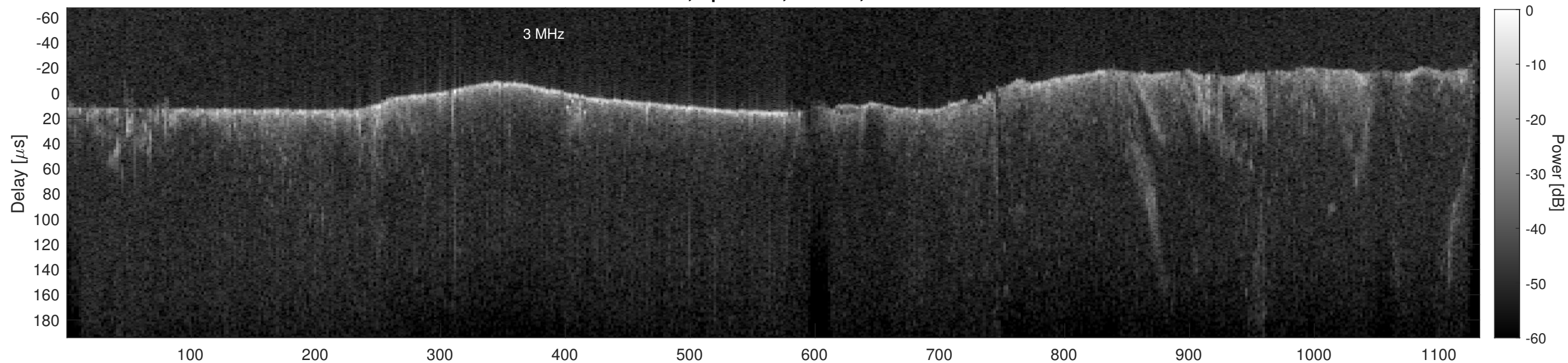
Orbit 13487, Cluttergram
