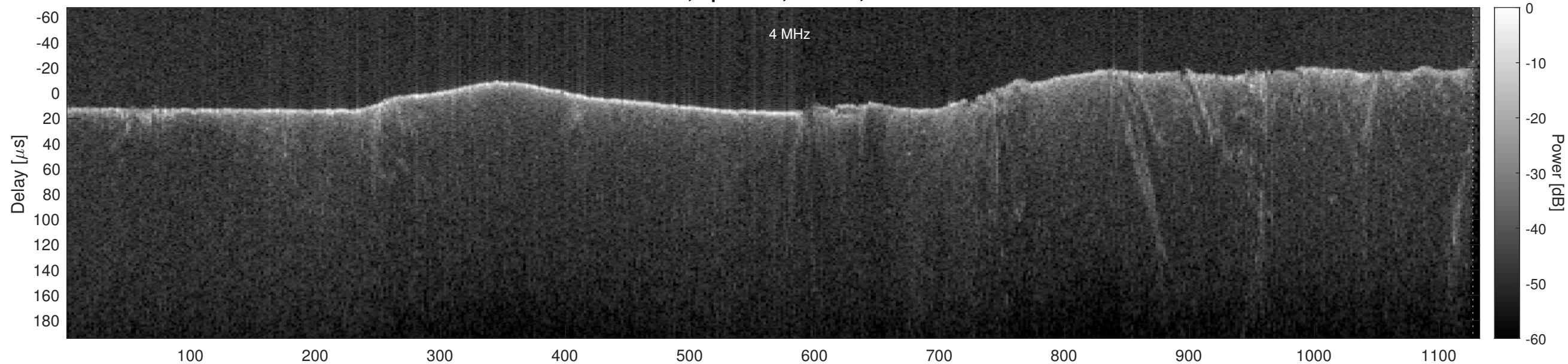
Orbit 13487, Optimized, Window, Channel 2
