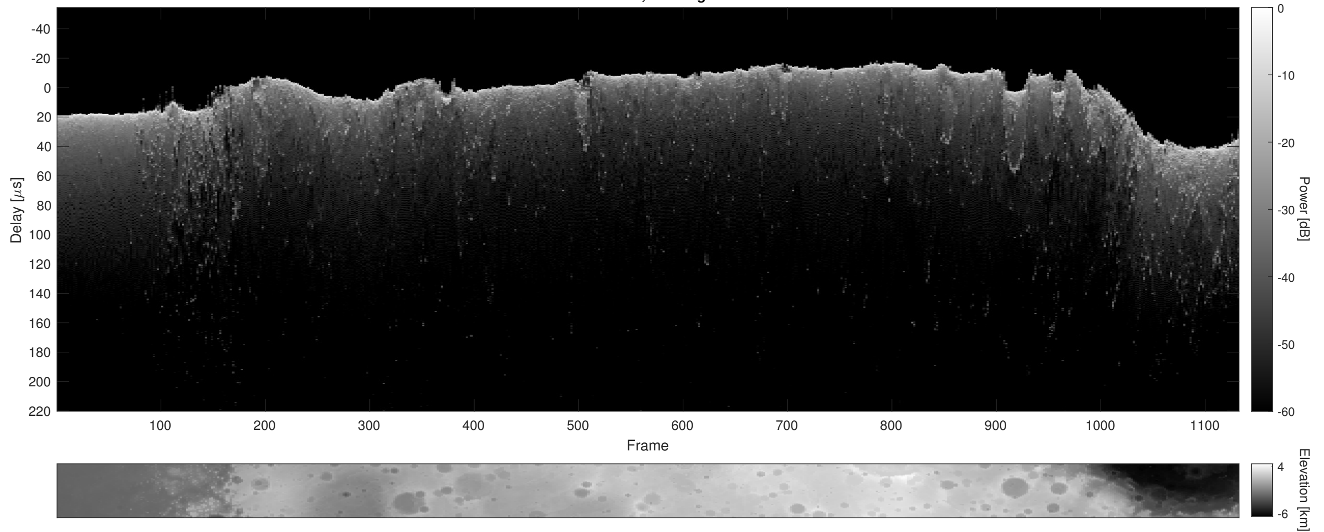
Orbit 13488, Cluttergram
