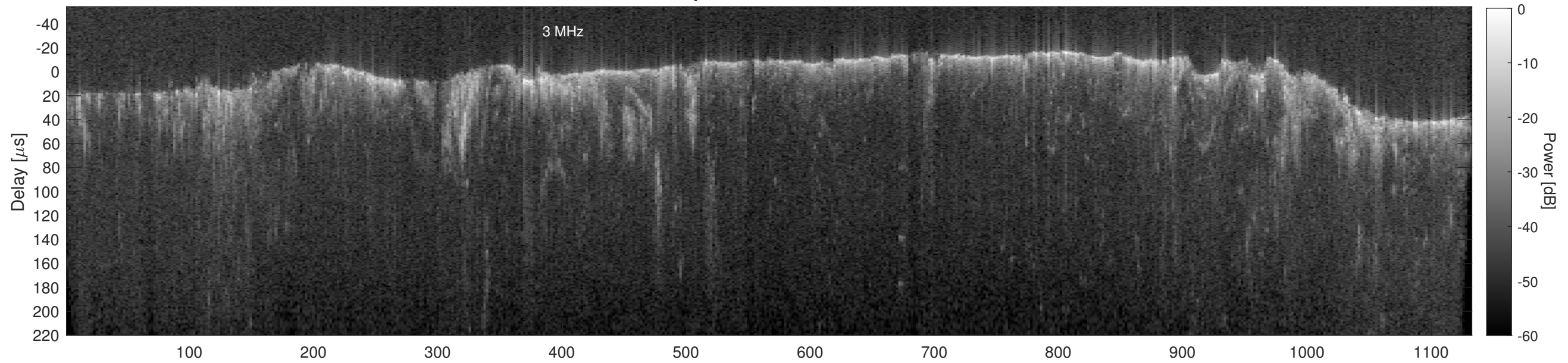
Orbit 13488, Cluttergram
