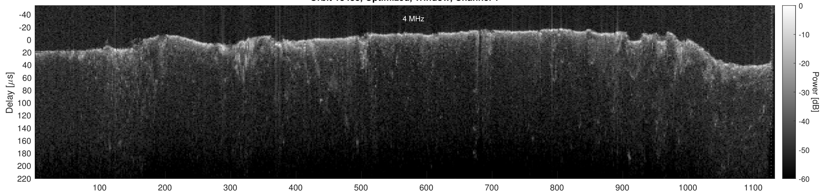
Orbit 13488, Optimized, Window, Channel 2
