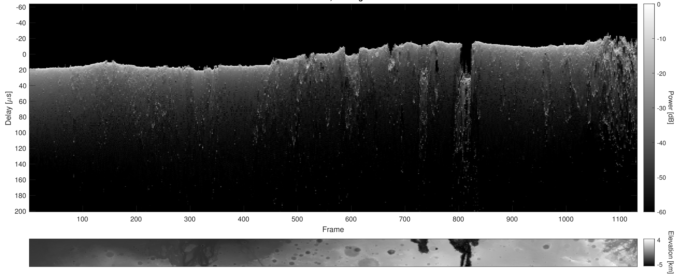
Orbit 13489, Cluttergram
