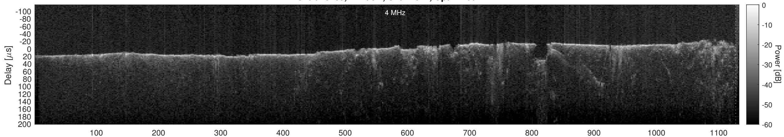
Orbit 13489, Cluttergram
