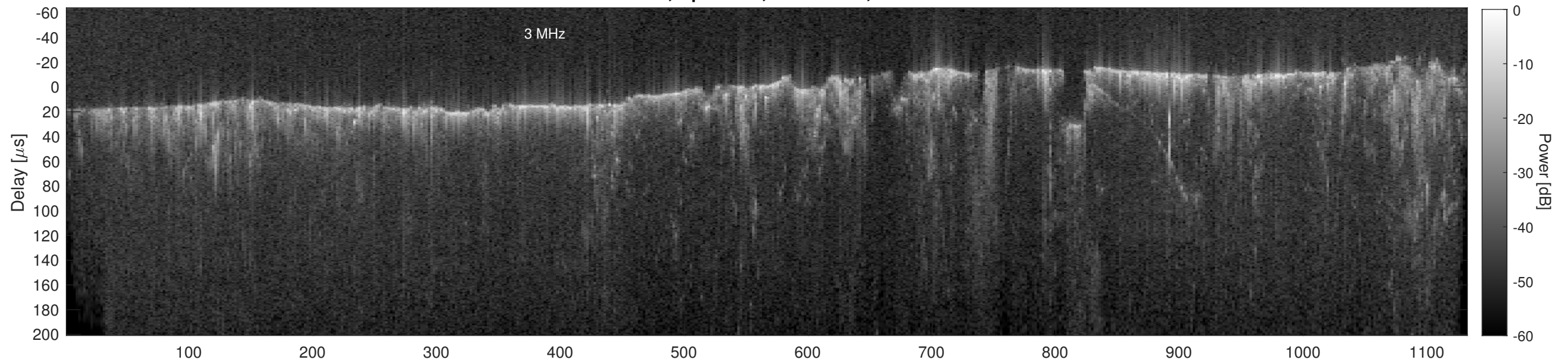
Orbit 13489, Cluttergram
