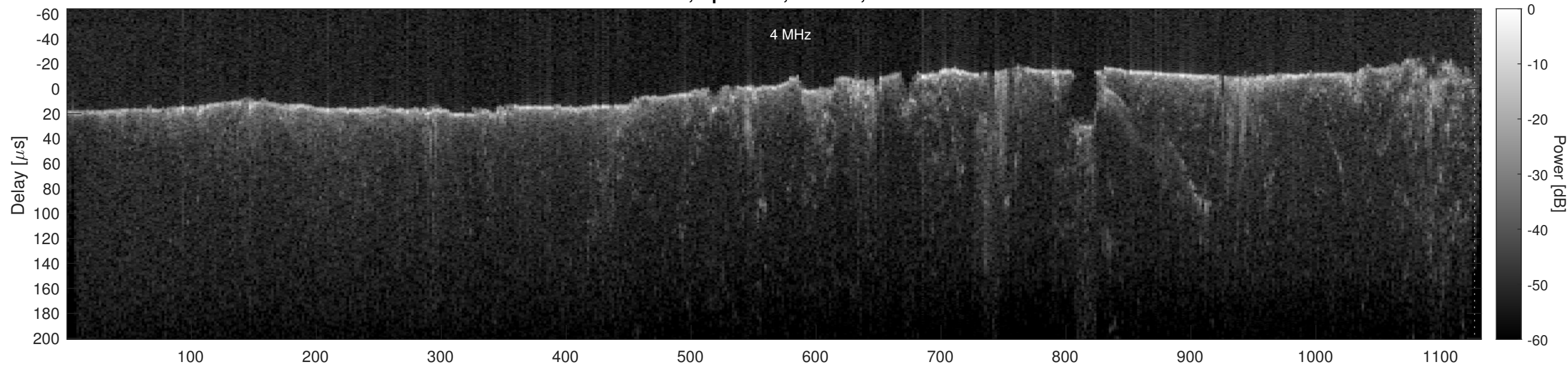
Orbit 13489, Optimized, Window, Channel 2
